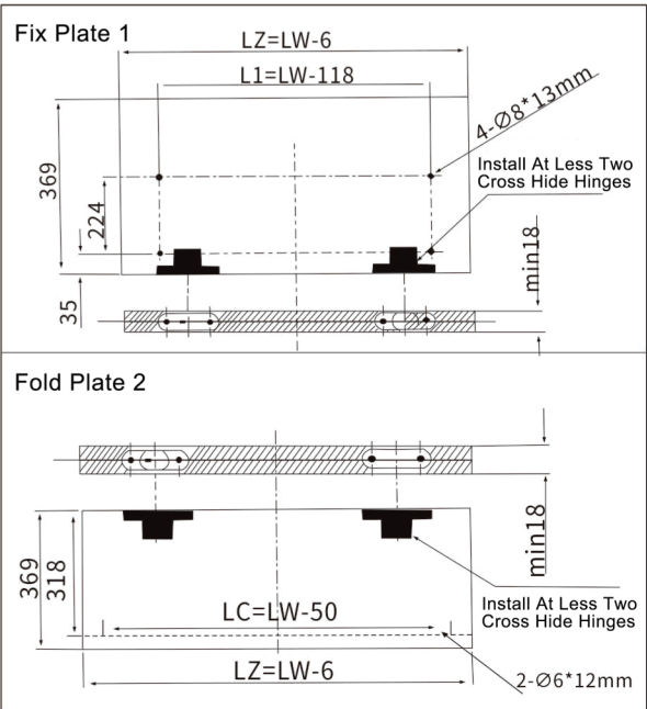
Fold Plate Detail(mm)
