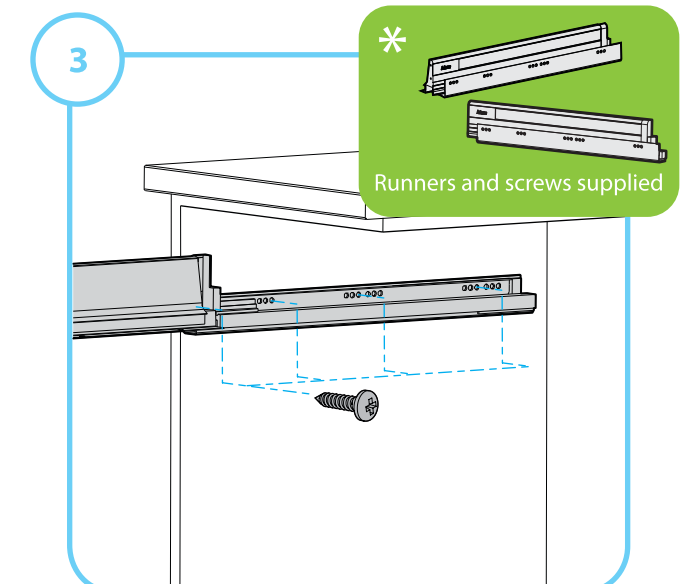
Mount runners as per manufacturer's instructions (runners and screws not supplied)
